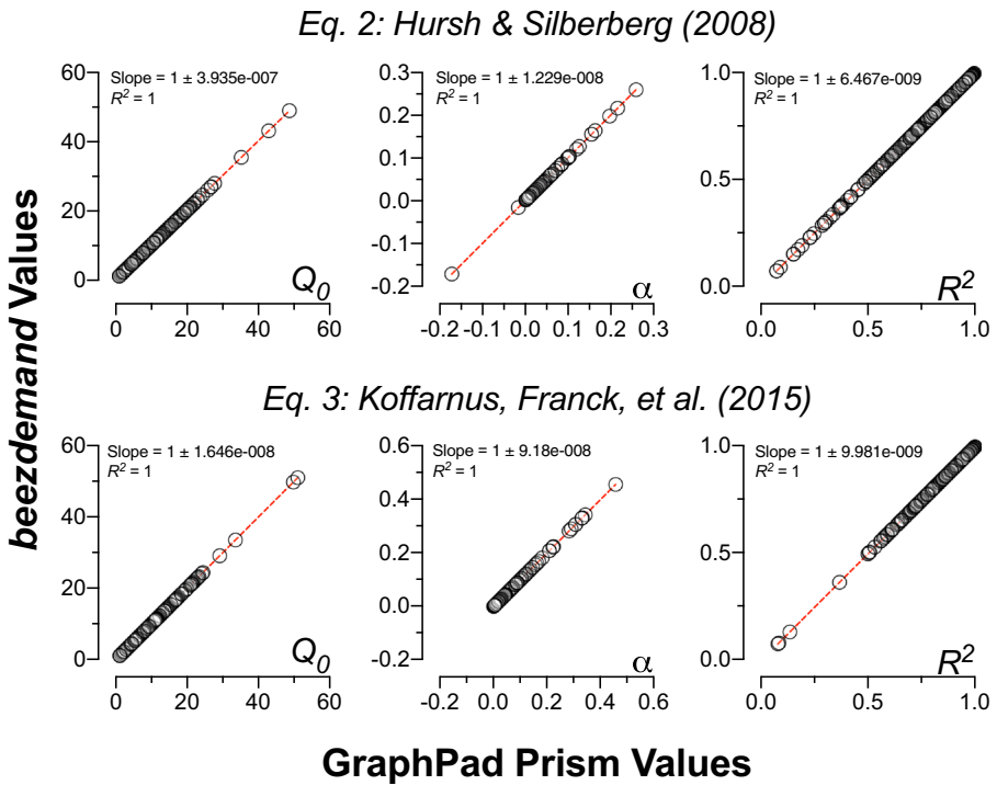
Fig. 3 Data from the empirical validation dataset. Correspondence in derived parameters from Equations 2 and 3 between beezdemand and GraphPad Prism™.
