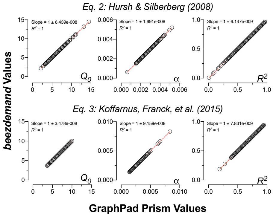
Fig. 2 Data from the simulated validation dataset. Correspondence in derived parameters from Equations 2 and 3 between beezdemand and GraphPad Prism™.
